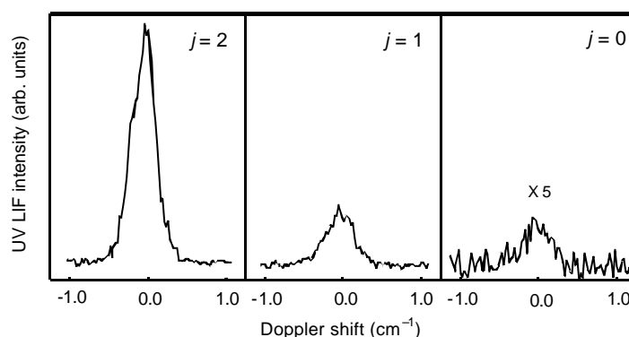
Figure 2. Vacuum ultraviolet LIF spectra of the O( 3 P j =2,1,0 ) atom products recorded 250 ns after pulsed (222.4 nm) excimer laser photolysis of 50 mTorr of SO 2 . Line centers correspond to the (3 s 3 S° ← 2 p 3 P j )-transition of the O( 3 P j =2 ), O( 3 P j =1 ) and O( 3 P j =0 ) atom fragments at 76794.98 cm -1 , 76636.72 cm -1 and 76568.00 cm -1 respectively.
